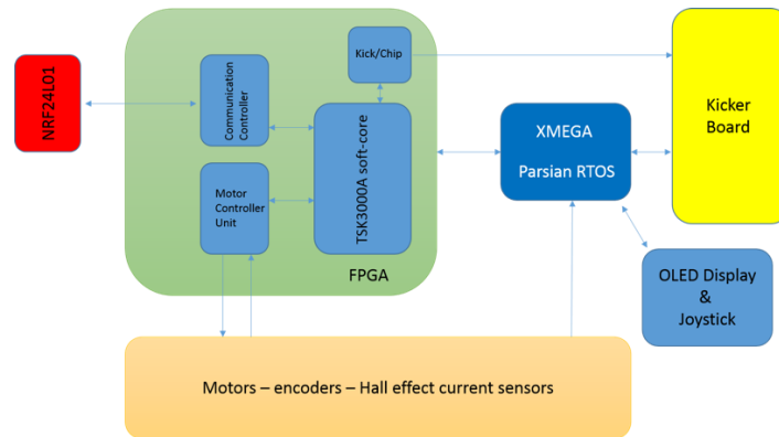
Fig. 4. New Main-Board Block Diagram
