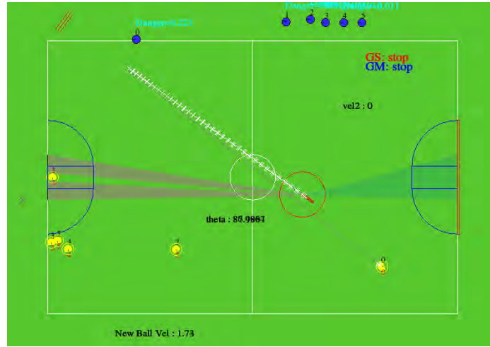
Fig. 7. Search ball path to find the best point to intercept ball
